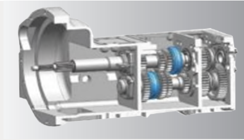
12+12 shuttle gears
