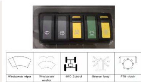
Electro Hydraulic Control 4WD and PTO
